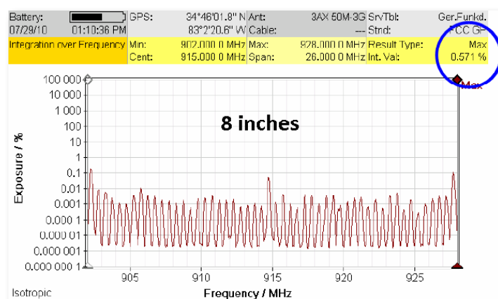
Figure 7 – Readouts of exposure levels at 8 inches behind the rack. Note that the exposure levels are expressed as a percentage of the FCC limit (circled in blue).
